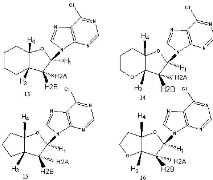
FIGURE 2 Relative stereochemistry of nucleosides 13–16.
