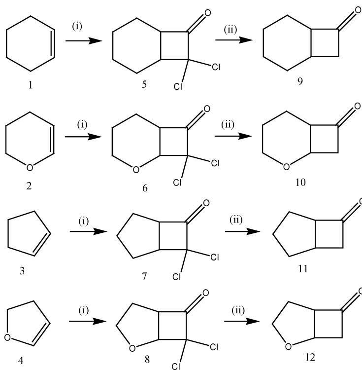
SCHEME 1 [2+2] cycloaddition.
