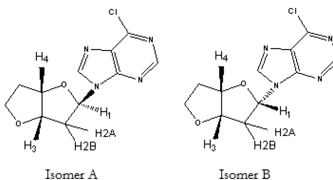
FIGURE 4 Two isolated isomers of nucleoside 16.
