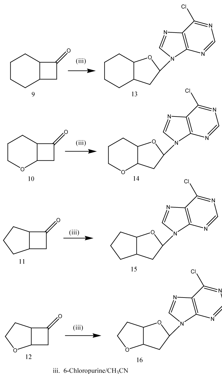
SCHEME 2 Photolytic ring expansion.
