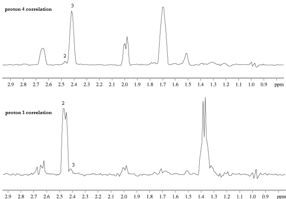
FIGURE 5 1D slice of 2D NOESY of nucleoside 13
