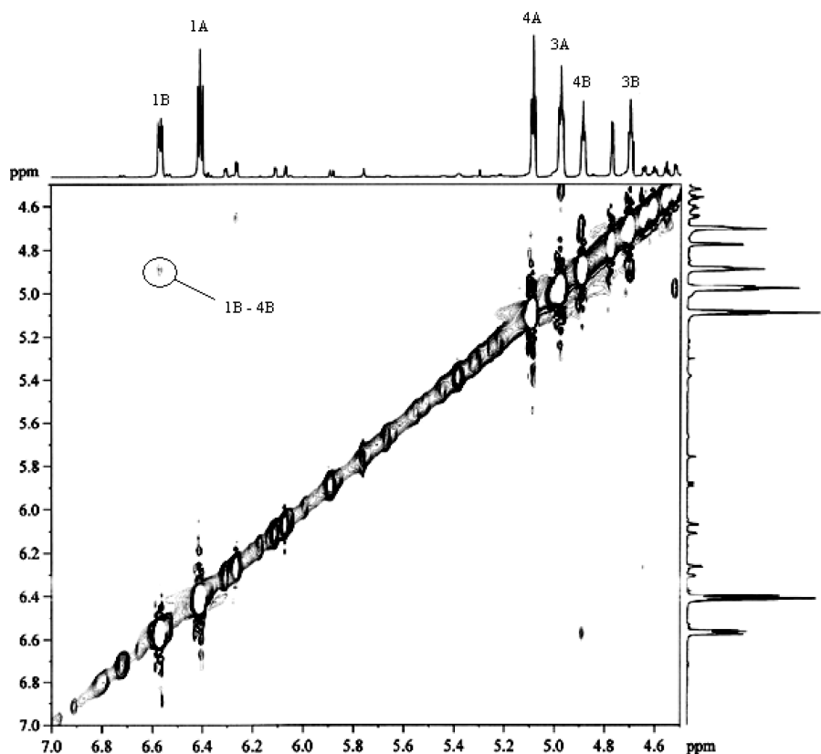
FIGURE 3 NOESY of isomers A and B of nucleoside 16.
