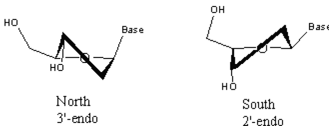
FIGURE 1 Conformations of ribonucleosides.
